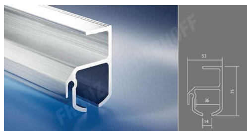
rail type b
